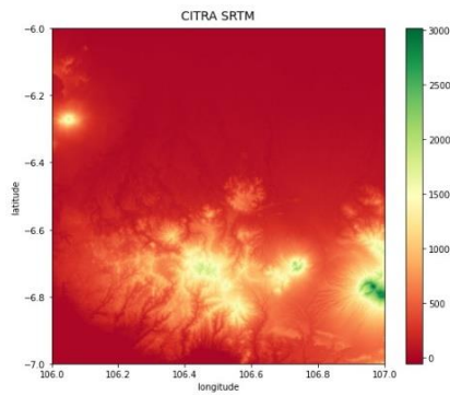
Gambar 3. Citra SRTM
