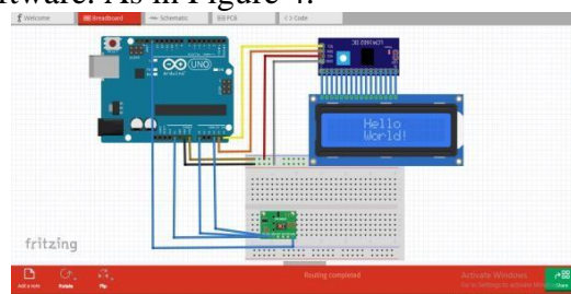
Figure 4. Electrical System Design
