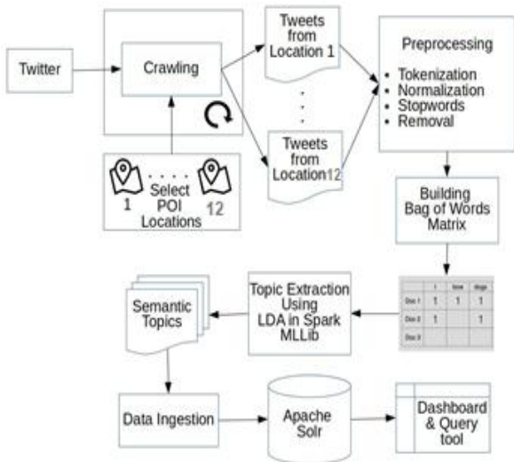
Fig. 1. Start to end diagram process to fetch insights from Twitter on top of proposed Big data platform
