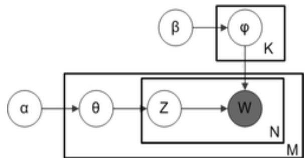
Fig. 2. Latent Dirichlet Allocation architecture
