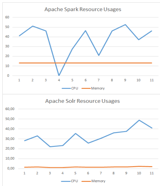
Fig. 4. Graphical resource (CPU and Memory) usages by Apache Solrand Apache Spark
