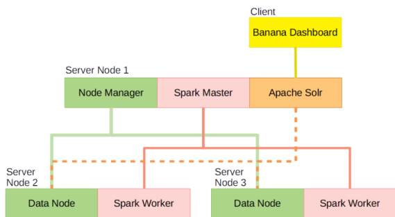
Fig. 3. The interaction between three main big data programs that deployed in the proposed platform
