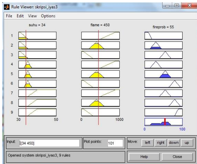
Gambar 4 Rule Viewer
