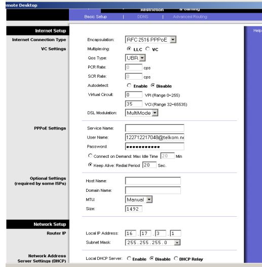
Fig. 5. IP Settings at the Branch Office
