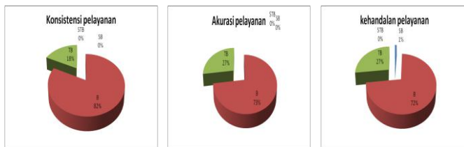
Gambar 4.6. Dimensi Reliability
