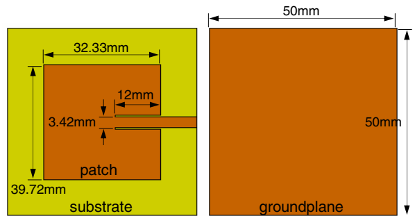
Fig. 4. Conventional patch antenna for investigation of size reduction.
