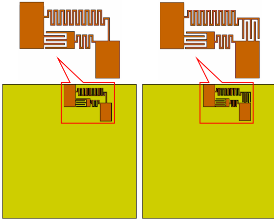
Fig. 2. Matching circuit designed using IDC and MI on top side of second layer; left is Type 1; right is Type 2.
