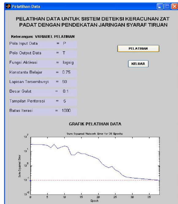
Gambar 5. Form Pelatihan Data
