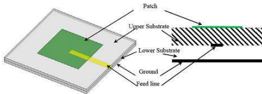
Gambar 2.13 Proximity Coupled Feeding
