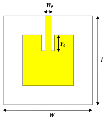
Gambar 3.3. Antena Konvensional
